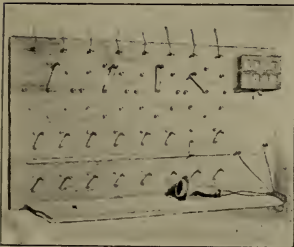
THE FIRST TELEPHONE SWITCHBOARD USED IN NEW HAVEN, CONN., FOR EIGHT SUBSCRIBERS
